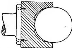
FIG. 330. CHUCKING A SPHERE —FIRST METHOD.
